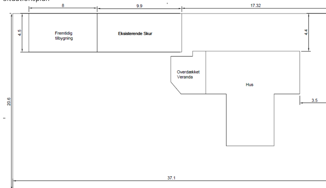
Situationsplan
